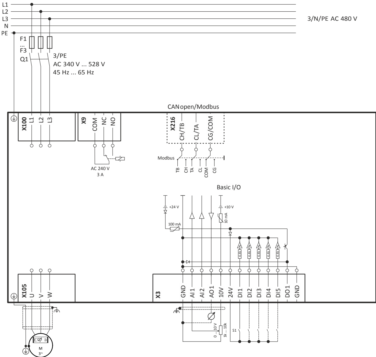
Fig. 8: Wiring example
